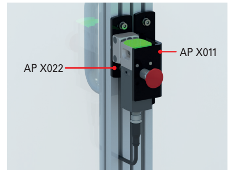
Hinged doors, with switch installed on the inside of the door.
